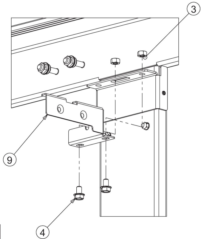
Welded Centerpost
